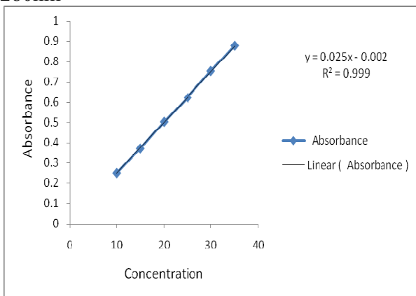
Figure 3.1 Citicoline accuracy and linearity on 280nm
