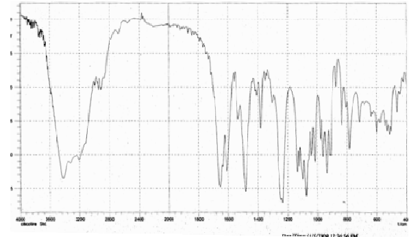
Figure 3.2 IR spectrum of Citicoline standard
