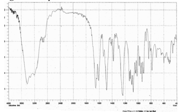
Fig.3.3 IR spectrum of Citicoline tablet
