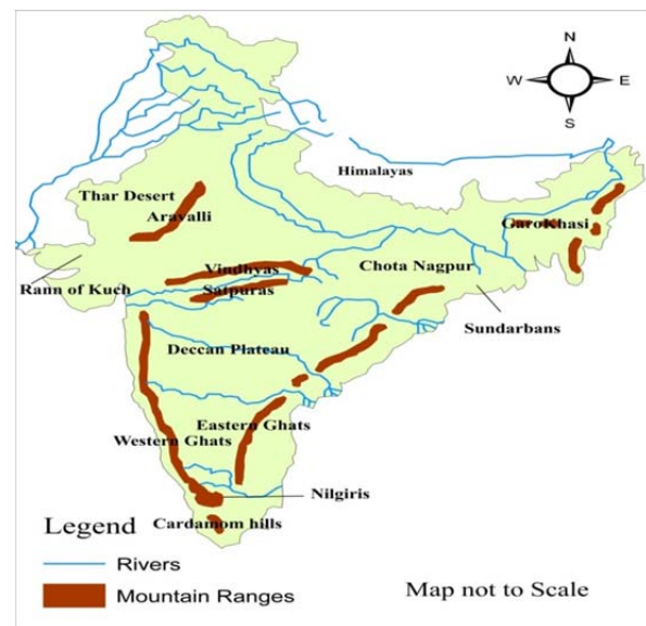
Fig. 1: The mountain ranges of peninsular India
